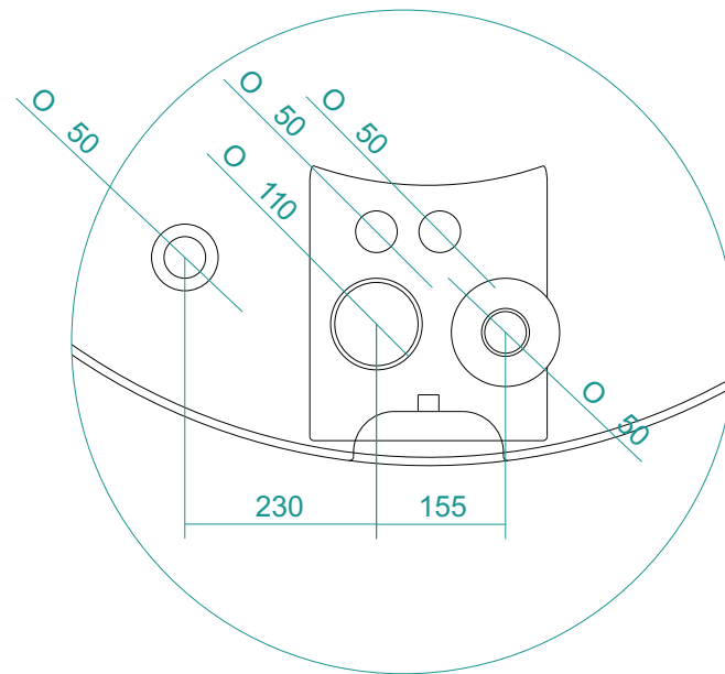
DETAIL A
